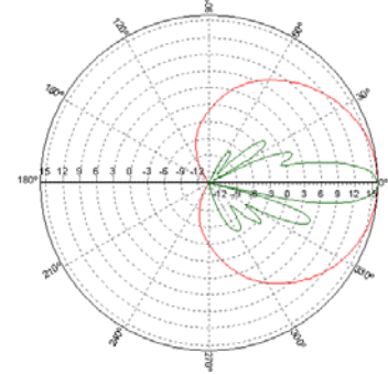
Typical Horizontal and Vertical 7329.00 Patterns 925 MHz
